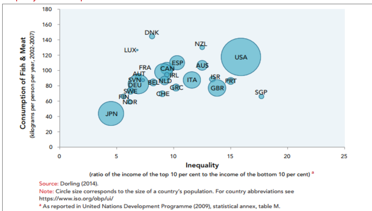
Figure 5 Inequality and consumption of fish and meat across countries
