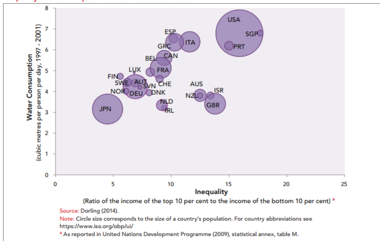
Figure 4 Inequality and consumption of water across countries
